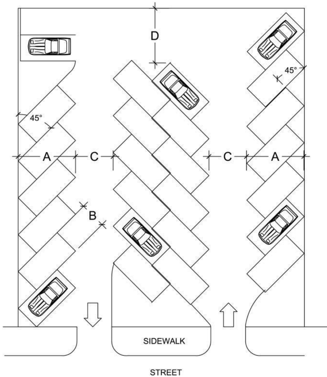
45 DEGREE PARKING LAYOUT (36-58b.1)
